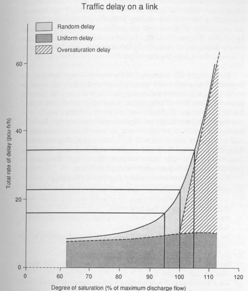
Figure A4.1 The effects of increases in traffic flow on congestion
